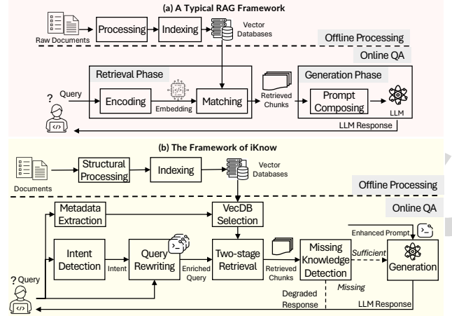
Fig. 6. The framework of iKnow compared to the existent system.
