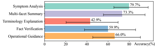
Fig. 3. Response accuracy of different intent types.
